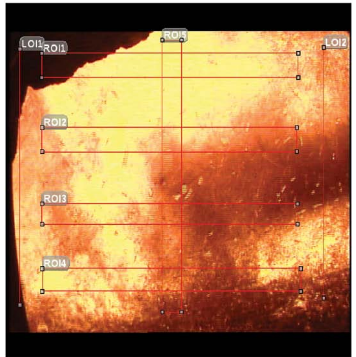
Thermography at grate-level vs CFD results of combustion gas temperature
